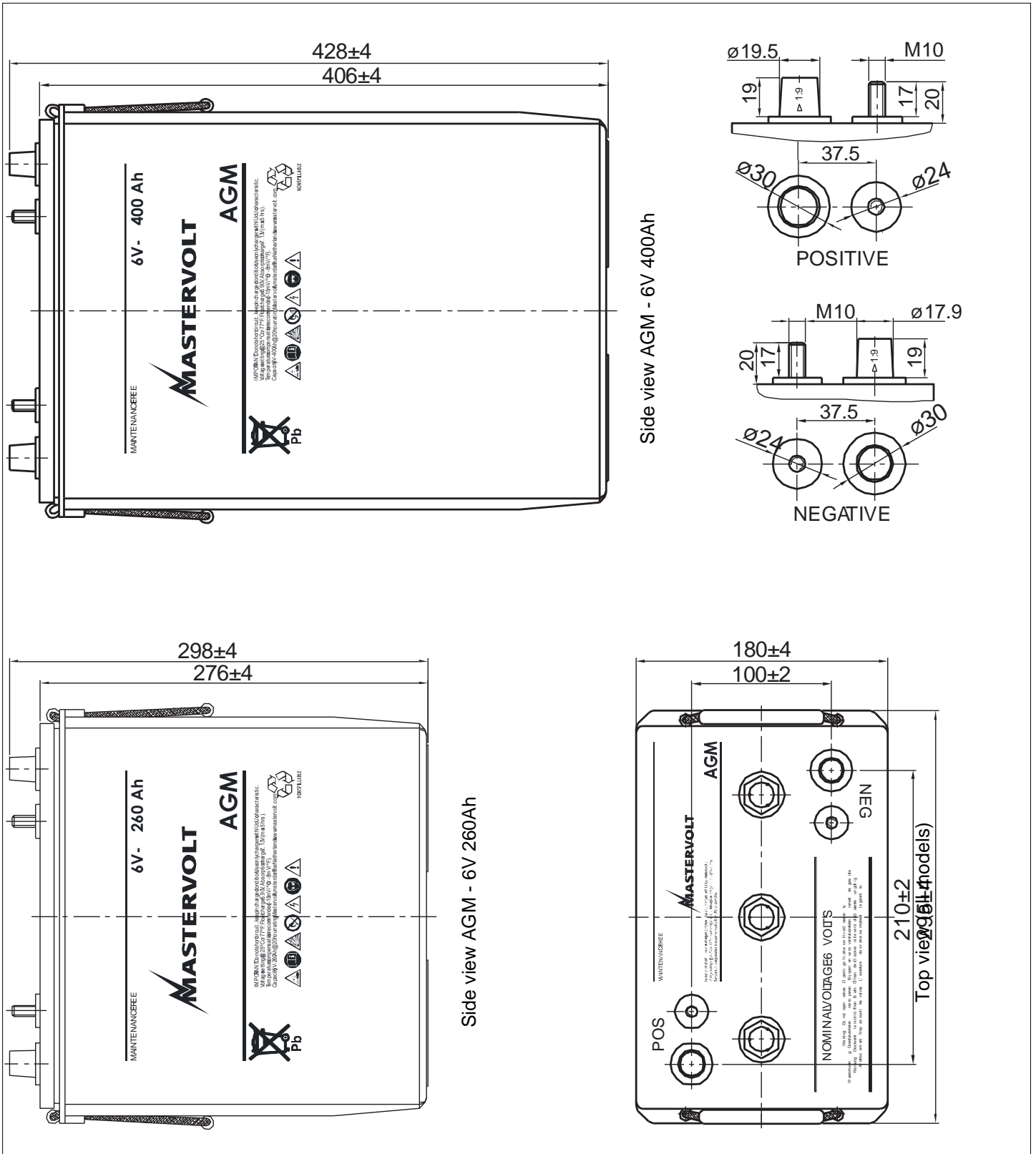
Figure 5: Dimensions in mm. See www.mastervolt.com/batteries for detailed drawings.
